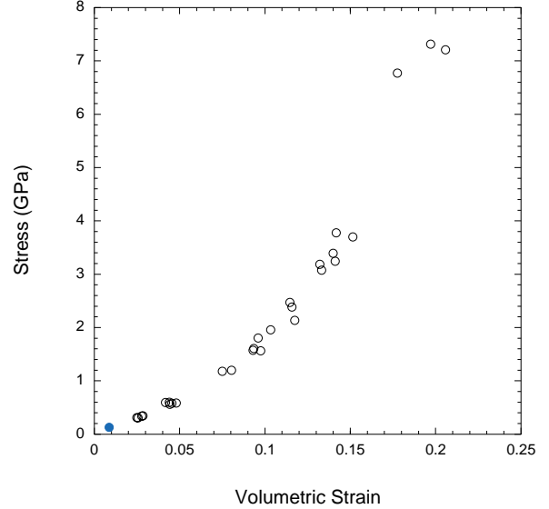
Figure 5: Longitudinal stress vs volumetric strain for PBX 9501. The volumetric strain is 1 - V/V_0 .
